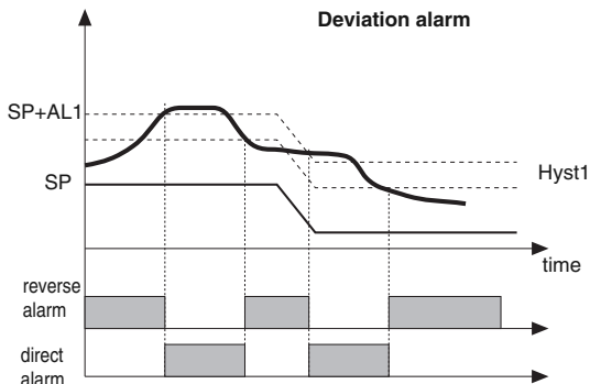
Deviation alarm
